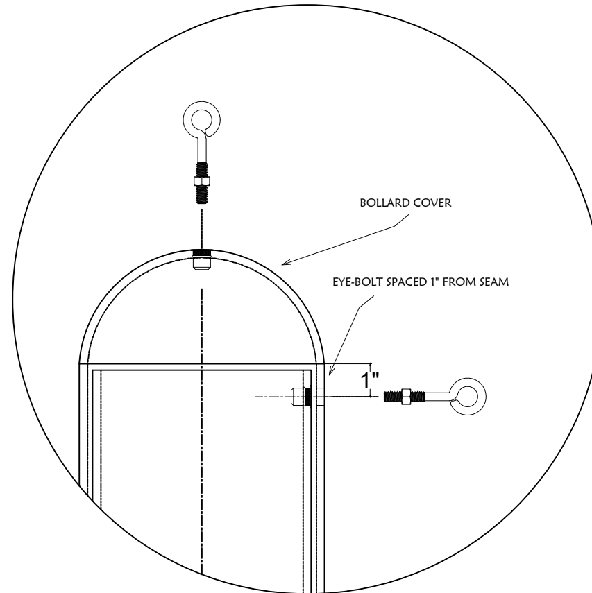
NEW PIPE BOLLARD AND SLEEVE ASSEMBLY
