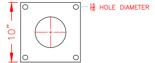
5/8" x 10" x 10" BASEPLATE
