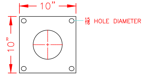
5/8X10X10 BASEPLATE
