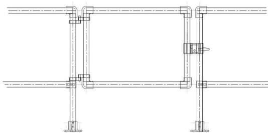
GATE WITH LATCH
