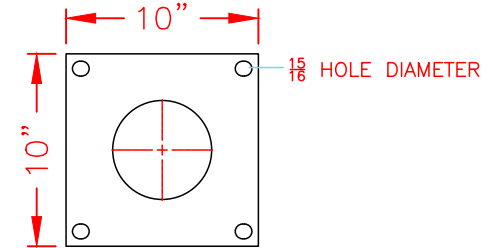
5/8X10X10 BASEPLATE
