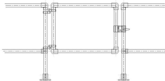
GATE WITH LATCH
