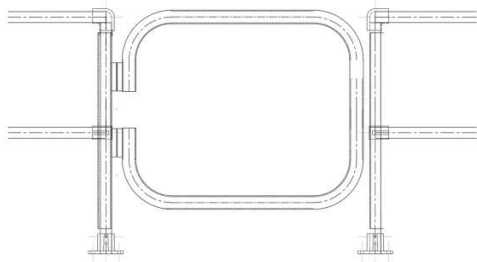
SELF CLOSING GATE
